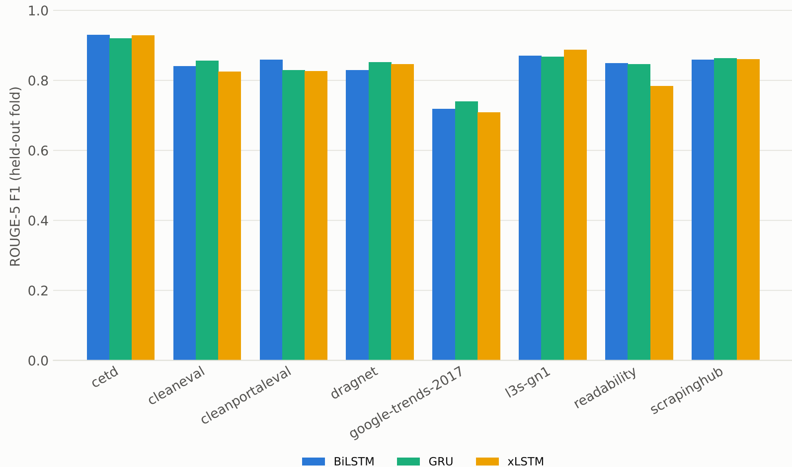
LODO per-fold ROUGE-5
