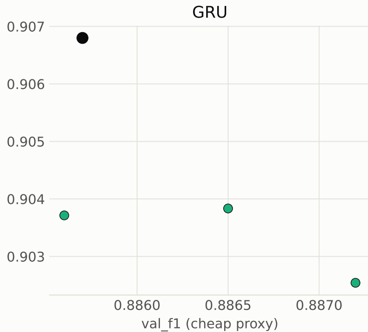
Sweep top-K: cheap proxy metric vs. real WCEB score (black = eventual winner)
