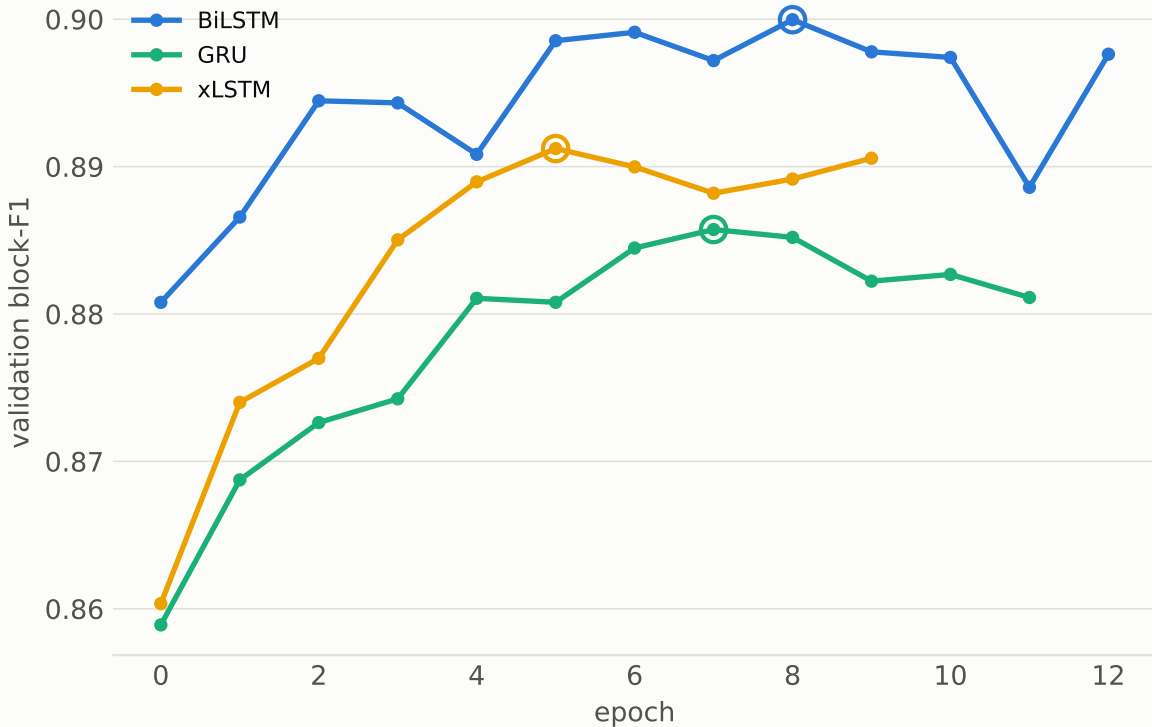
Training curves, winning config per architecture (open circle = checkpointed best epoch)
