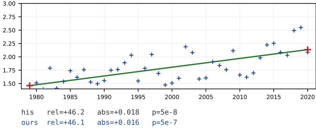
Brown energy dissipation rate (f)
