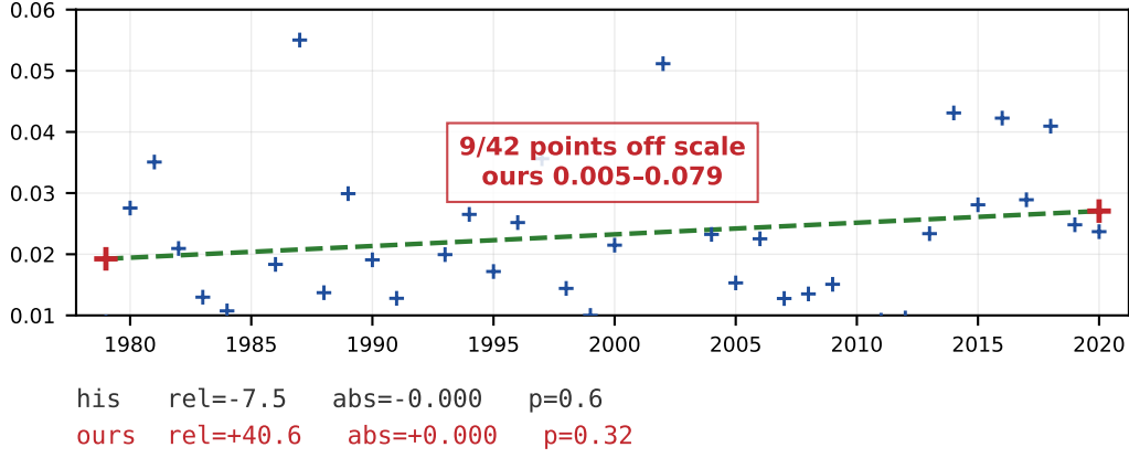
Negative Richardson number (a)
