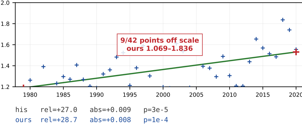
Variant 2 of Ellrod's turbulence index (h)
