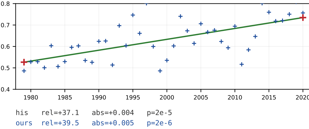
Relative vorticity squared (k)
