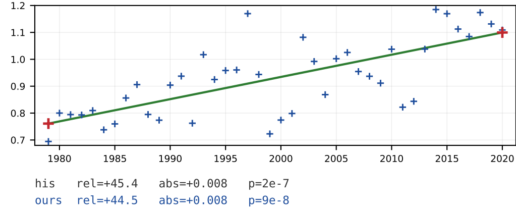
Brown index (e)
