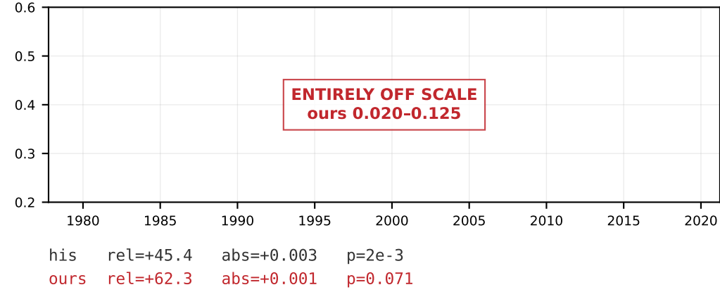
Colson-Panofsky index (c)
