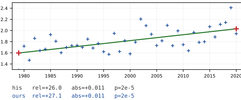
Magnitude of horizontal temperature gradient (l)
