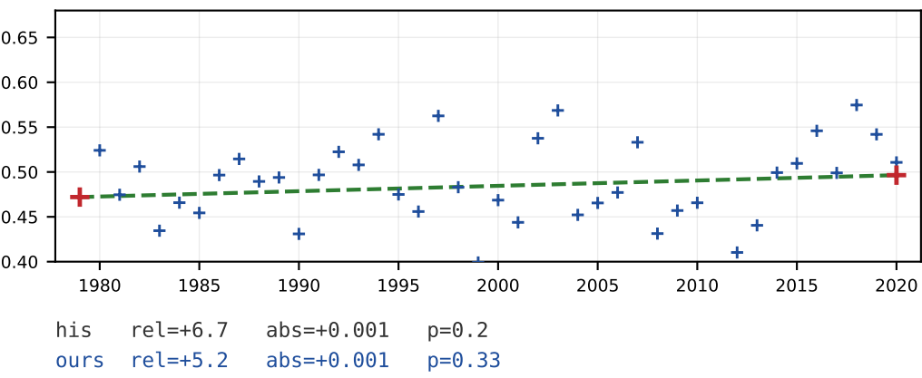
Magnitude of horizontal divergence (r)
