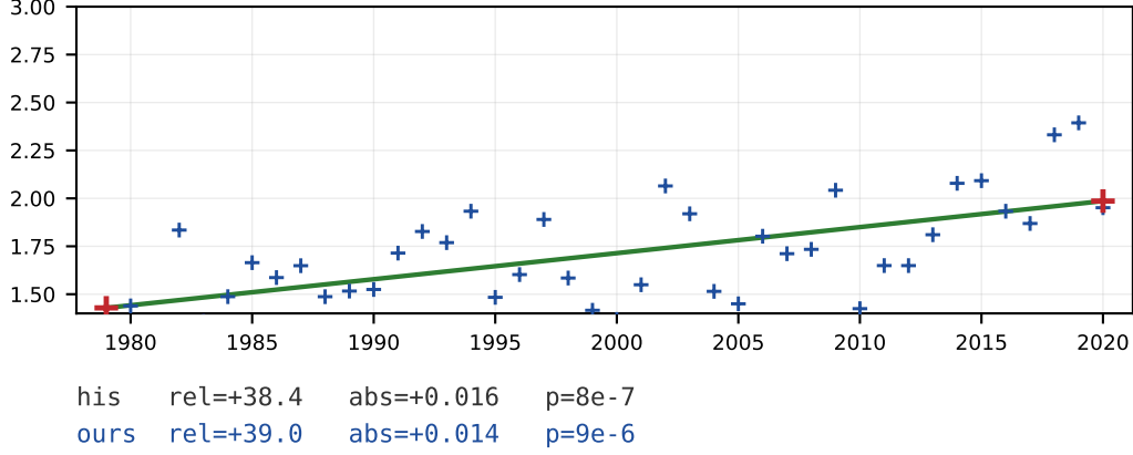
Magnitude of vertical shear of horizontal wind (b)
