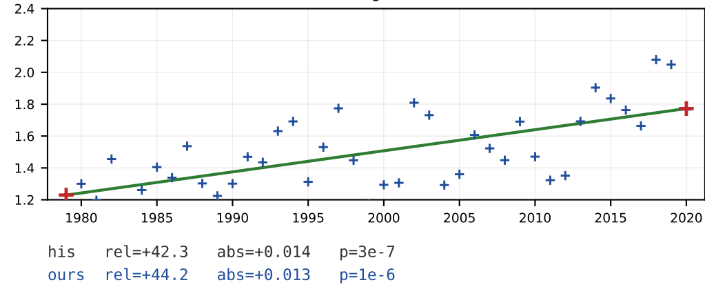
Variant 1 of Ellrod's turbulence index (g)
