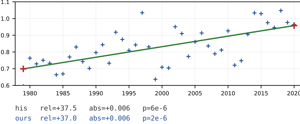
Flow deformation (i)
