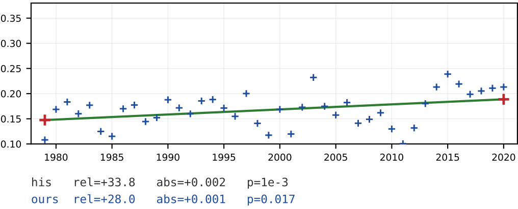
Flow deformation times vertical temperature gradient (p)
