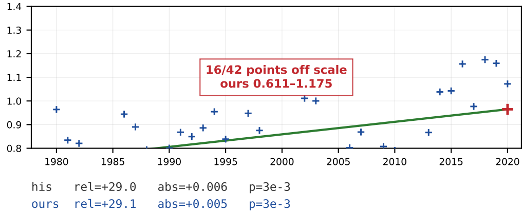
Magnitude of relative vorticity advection (u)
