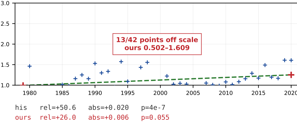
Magnitude of potential vorticity (j)
