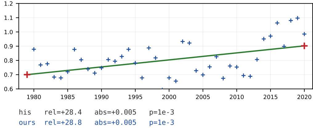
Negative absolute vorticity advection (t)
