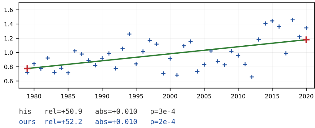
Flow deformation times wind speed (o)
