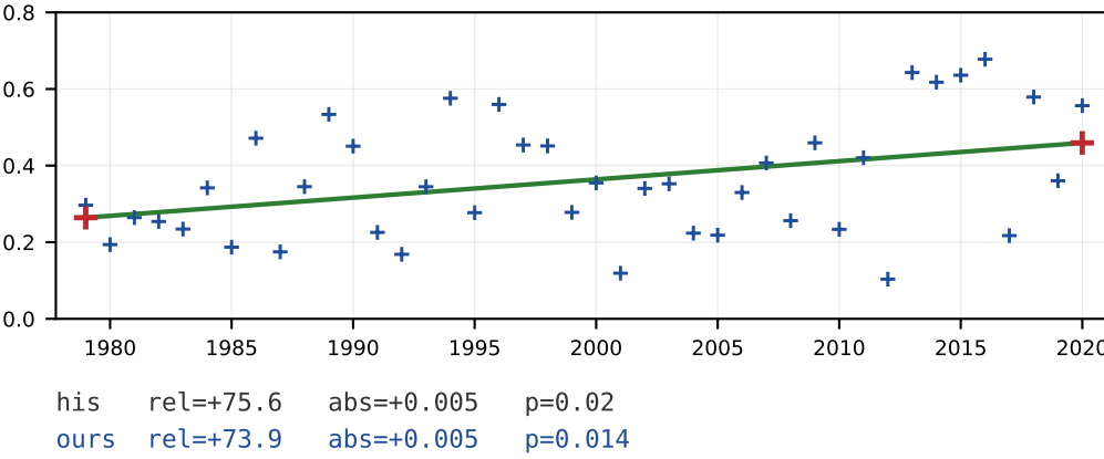
Wind speed (m)
