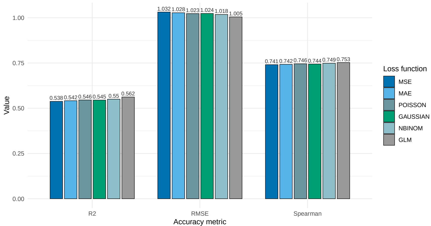
Model accuracy, intercept 6
