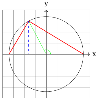
Figure: A random tikz graph
