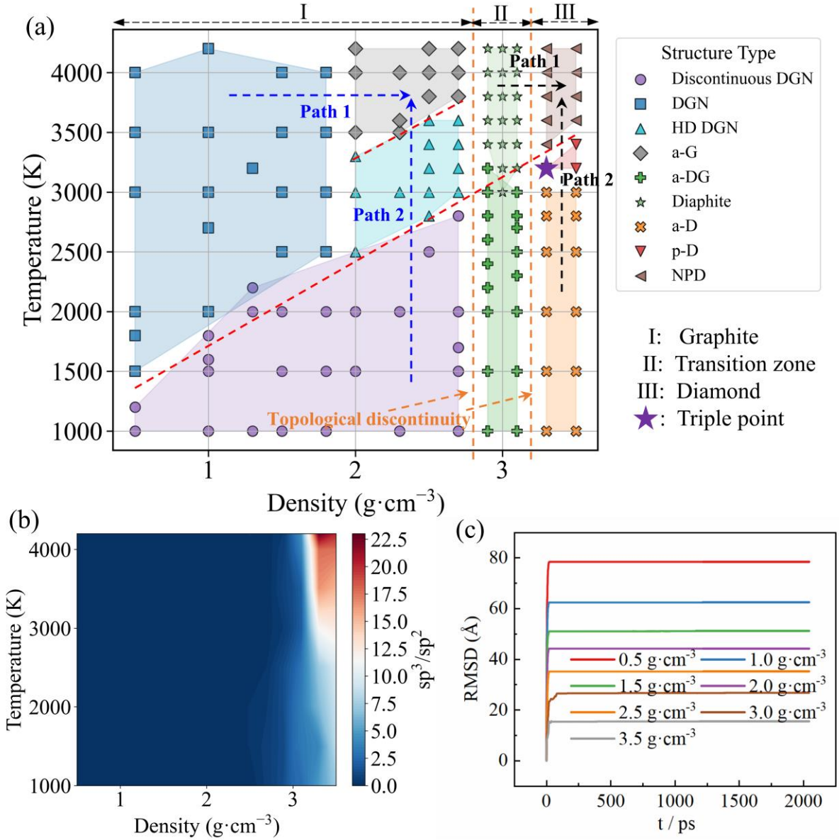
Fig. 4 Structural evolution of amorphous carbon under varying temperature and density conditions.
