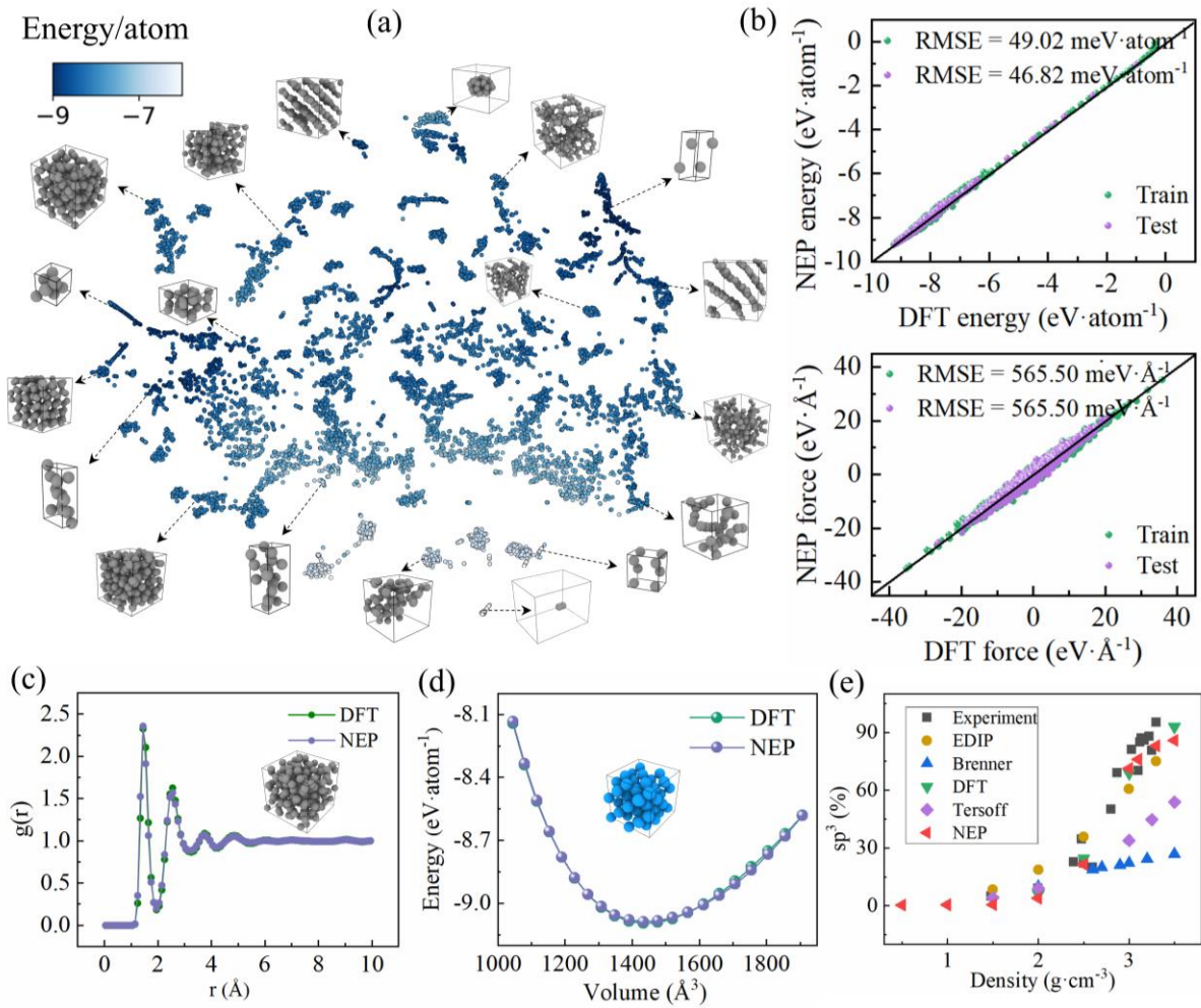
Fig. 1 Training and validation results of the NEP. (a) A schematic visualization of the dataset, where each point represents a carbon structure and is colored based on its average atomic energy. (b) Training results for energy (top) and forces (bottom). (c) Comparison of RDF obtained from 15 ps isothermal simulations at 4000 K for a 216-atom amorphous carbon system, driven by DFT and the NEP, respectively. (d) E - V curves of diamond structures under different strain conditions. (e) Comparison of sp^3 content in amorphous carbon prepared by different methods , showing good agreement between NEP, experimental data, and DFT results. Nine representative amorphous carbon structures
