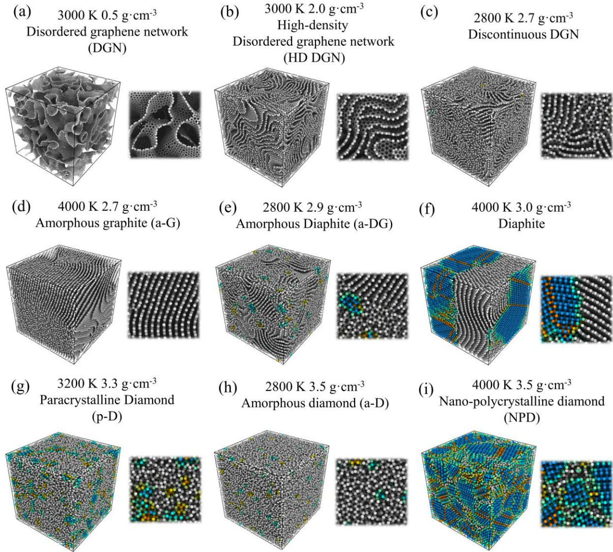
Fig. 2 Nine representative amorphous carbon structures formed under different temperature and density conditions. (a) DGN; (b) HD DGN; (c) Discontinuous DGN; (d) a-G; (e) a-DG; (f) Diaphite; (g) p-D; (h) a-D; (i) NPD. Atomic coloring is based on the “Identify Diamond Structure” function in OVITO 61 , with local magnified views shown alongside each structure. Detailed color classification is illustrated in supplementary Fig. 4 .
