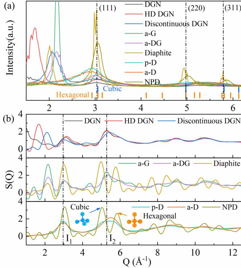
Fig. 3 Identification of nine different amorphous carbon structures. (a) Calculated XRD patterns, with short vertical lines below the curves indicating the diffraction peak positions of cubic and hexagonal diamond. (b) Structure factor.
