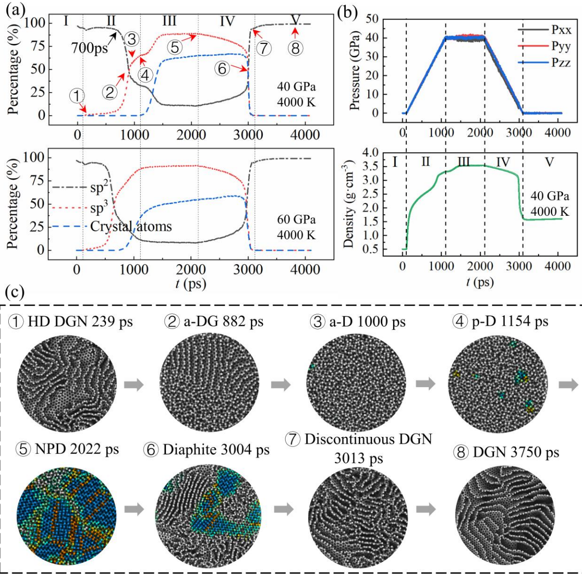
Fig. 5. Phase transitions between different amorphous carbon. (a) Evolution of sp^2 , sp^3 , and crystalline atom fractions during annealing under two target pressures, 40 GPa and 60 GPa. Crystalline atoms are defined as the sum of cubic and hexagonal diamond atoms, excluding first and second nearest neighbors. Stage I: Initial relaxation of the DGN structure at 4000 K for 100 ps; Stage II: Temperature held at 4000 K while pressure is gradually increased to 40 GPa over 1000 ps; Stage III: System relaxed at 4000 K and 40 GPa for an additional 1000 ps; Stage IV: Temperature maintained at 4000 K while pressure is released to 0 GPa; Stage V: Temperature reduced to 300 K under 0 GPa. (b) Time evolution of system pressure and density under the 40 GPa target pressure. (c) Structural snapshots at key time points during the phase transition, corresponding to the 40 GPa, 4000 K conditions shown in (a).
