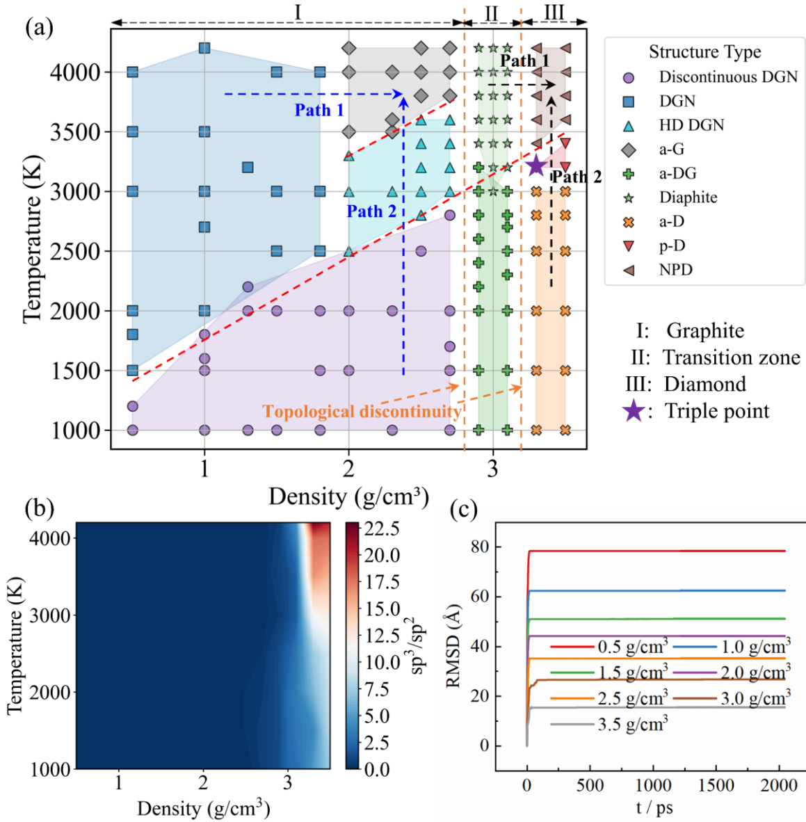
Fig. 4 (a) Temperature–density phase diagram of amorphous carbon. (b) Distribution map of the sp^3/sp^2 ratio formed under different temperature and density conditions. (c) Time evolution of the RMSD during isothermal annealing at 3000 K for amorphous carbon structures with varying densities.
