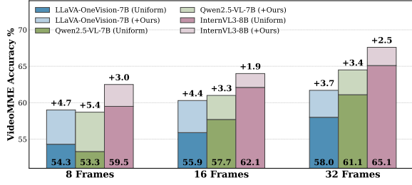
Figure 5: Video-MME accuracy under different frame budgets ( K \in \{8, 16, 32\} ) for three LVLM backbones. AGE-Sampler maintains stable gains across frame budgets, further validating its robustness on benchmarks with diverse video lengths and question types.
