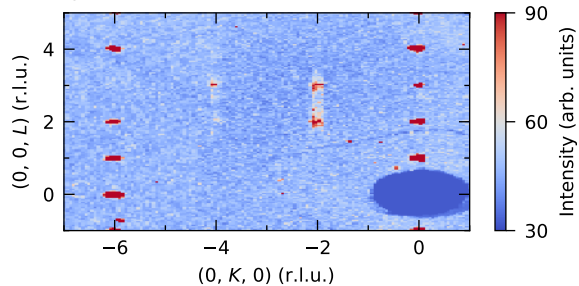
XRD, 300 K
