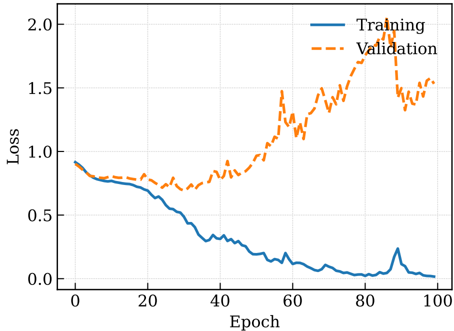
Training & Validation Loss
