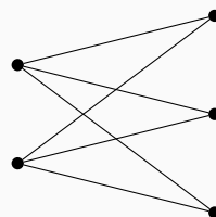
K_{2,3}
