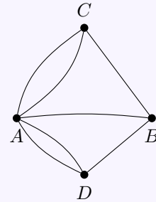
Abstract graph G
