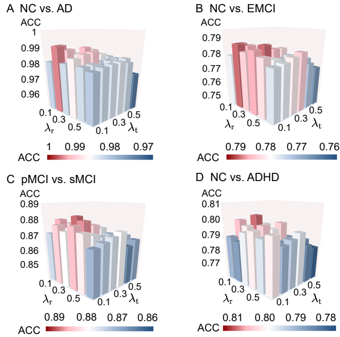
Figure S2: Comparison of hyperparameters for RRI thresholding.
