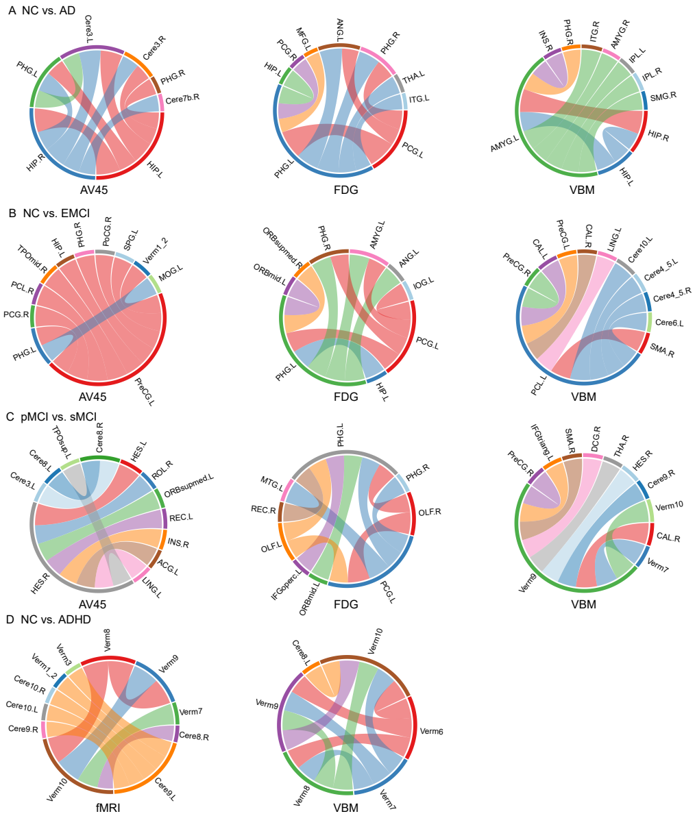
Figure S5: Region-level pairwise ablation analysis within individual modalities for intra-modality interaction patterns in (A) NC vs. AD, (B) NC vs. EMCI, (C) pMCI vs. sMCI, and (D) NC vs. ADHD tasks.
