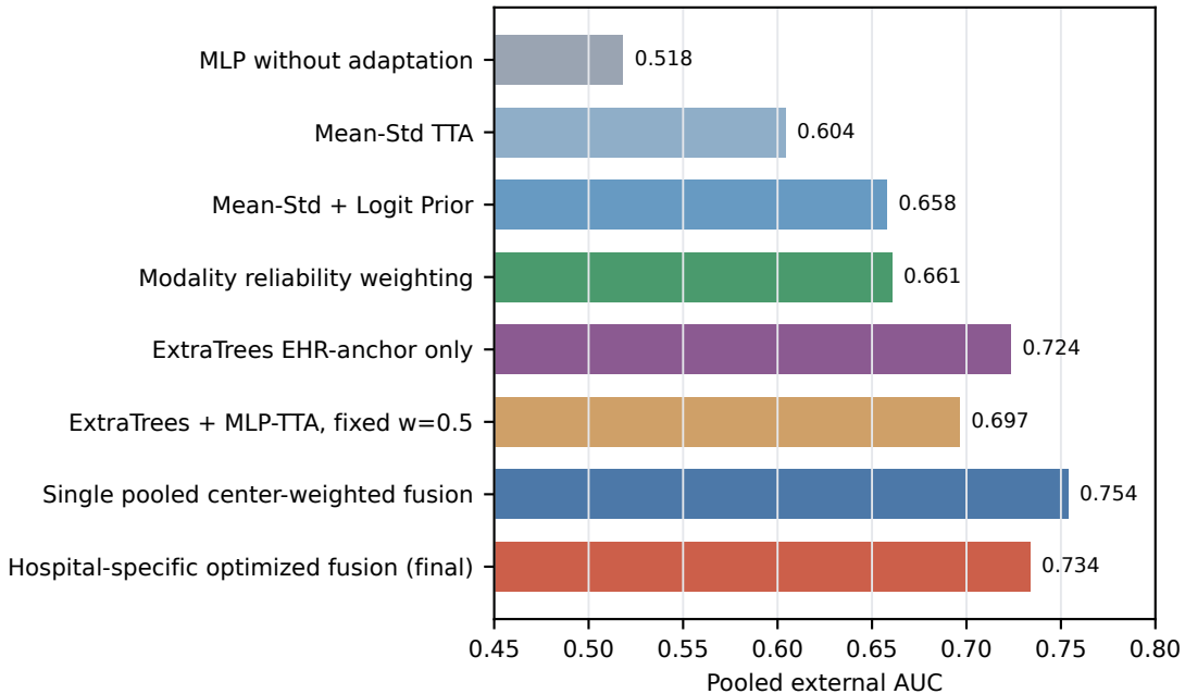
Effect of adaptation components
