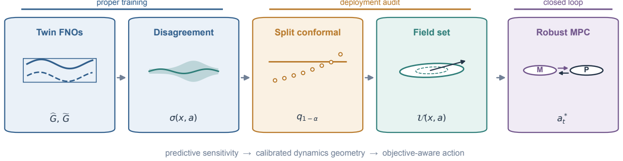
Figure 1: Uncertainty-to-control pipeline. Twin FNO predictions produce a spatial disagreement scale; split conformal calibration turns that scale into a field-valued dynamics set, which robust MPC queries inside the closed loop.
