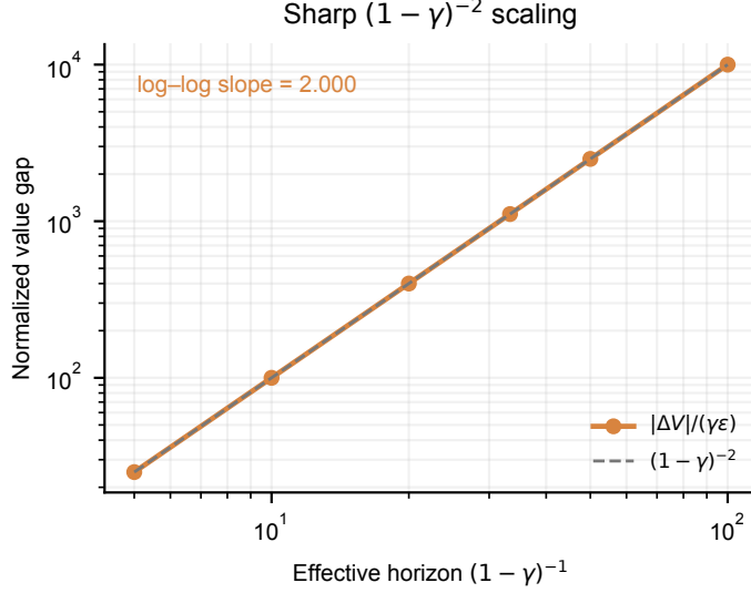
Figure 2: A sharp fixed-policy witness attains the O(\epsilon/(1 - \gamma)^2) rate. The plotted value gap is normalized by \gamma\epsilon , making the predicted slope exactly two. This is a theorem sharpness check, not a learned-model performance result.
