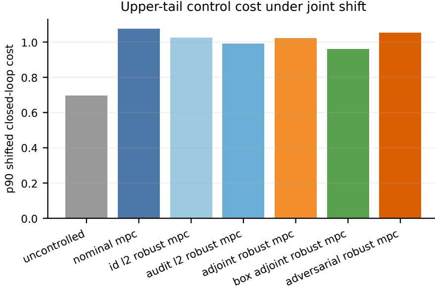
Figure 3: Empirical p_{90} closed-loop cost for the matched combined-shift actuator-gain sweep. The simultaneous-box adjoint controller gives the largest tail reduction, while the nonlinear adversarial controller is not best in this finite compute budget.
