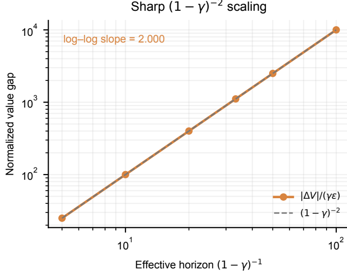
Figure 1: A sharp fixed-policy witness attains the O(\epsilon/(1 - \gamma)^2) rate. This verifies the exponent; it is not a learned-model performance result.
