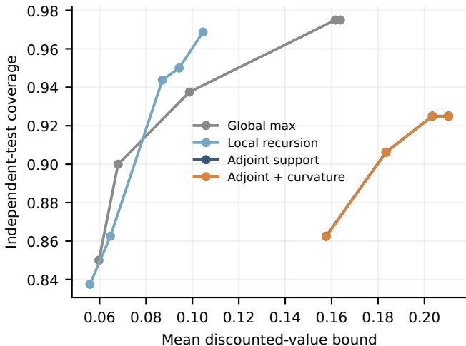
Coverage-conservatism frontier
