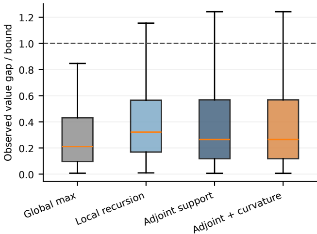
Independent-test utilization distribution
