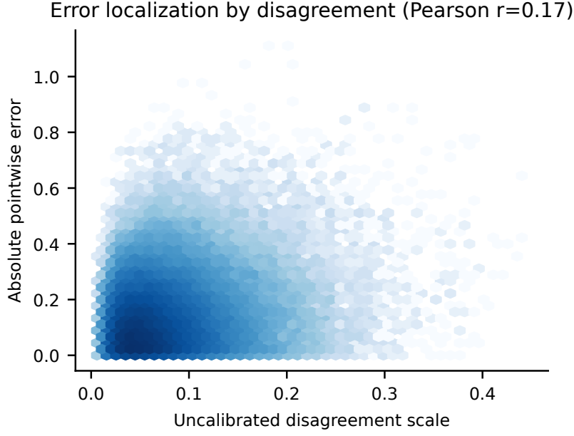
Figure 5: Pointwise perturbation scale versus absolute error on the independent Navier–Stokes test split. Pearson r = 0.169 reveals weak localization and helps explain the large simultaneous conformal multiplier.
