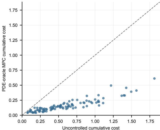
Paired task-validity comparison
