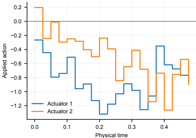
PDE-oracle MPC control input
