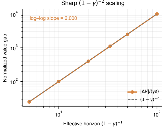
Figure 2: A sharp fixed-policy witness attains the O(\epsilon/(1 - \gamma)^2) rate. This verifies the exponent; it is not a learned-model performance result.
