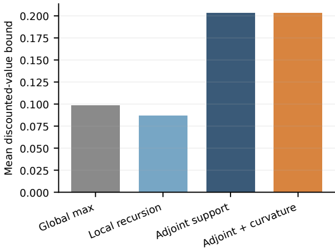
Bound conservatism at matched calibration
