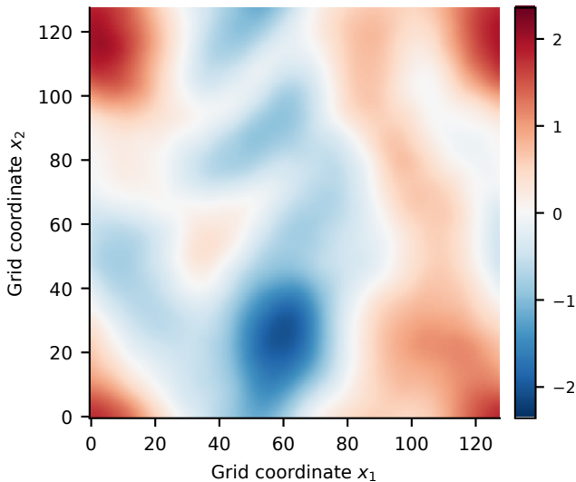
FNO prediction
