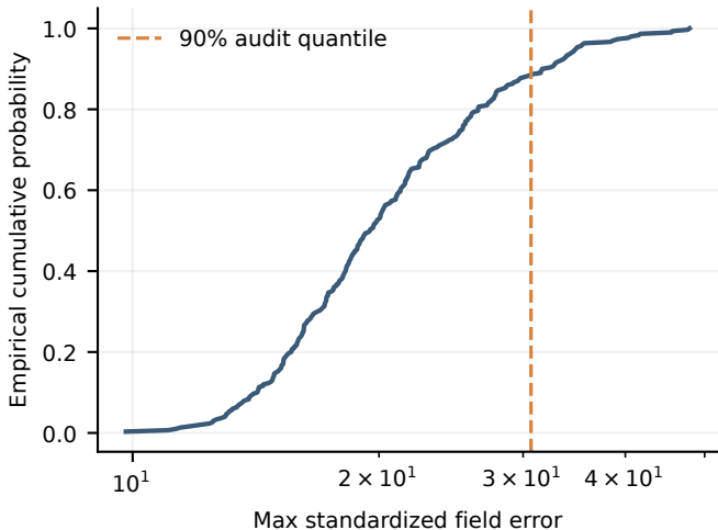
Simultaneous conformal score distribution
