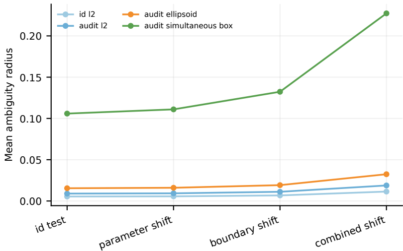
Ambiguity-set size under deployment shift
