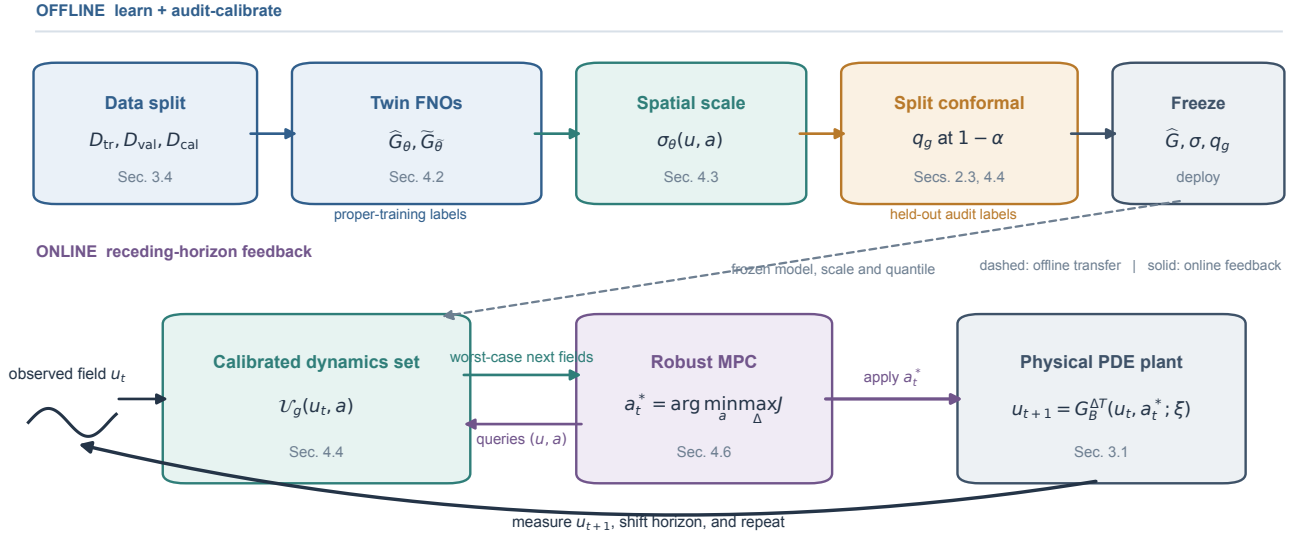
Figure 1: Closed-loop uncertainty-to-control architecture. Offline, the data roles in Section 3.4 feed the twin FNO, perturbation scale, and conformal calibration in Sections 4.2–4.5. Online, the calibrated field set is queried by the robust planner in Section 4.6. The selected action is applied to the controlled Burgers plant in Section 3.1, and the next observed field closes the receding-horizon loop. Dashed arrows denote offline transfer, not a claim that one-step marginal conformal coverage certifies the counterfactual closed loop.
