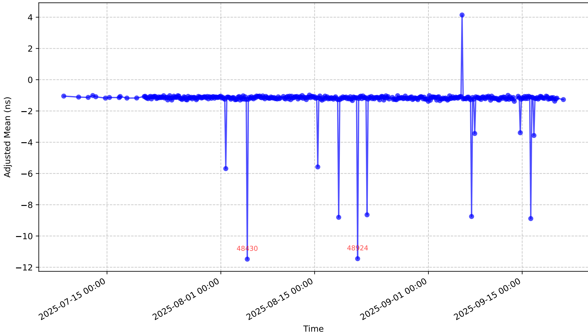
Channel 21 - Adjusted Mean Value Variation
