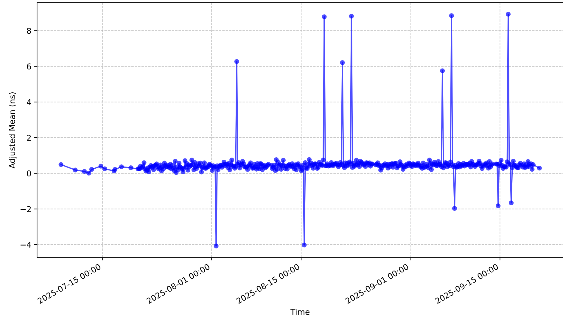
Channel 53 - Adjusted Mean Value Variation
