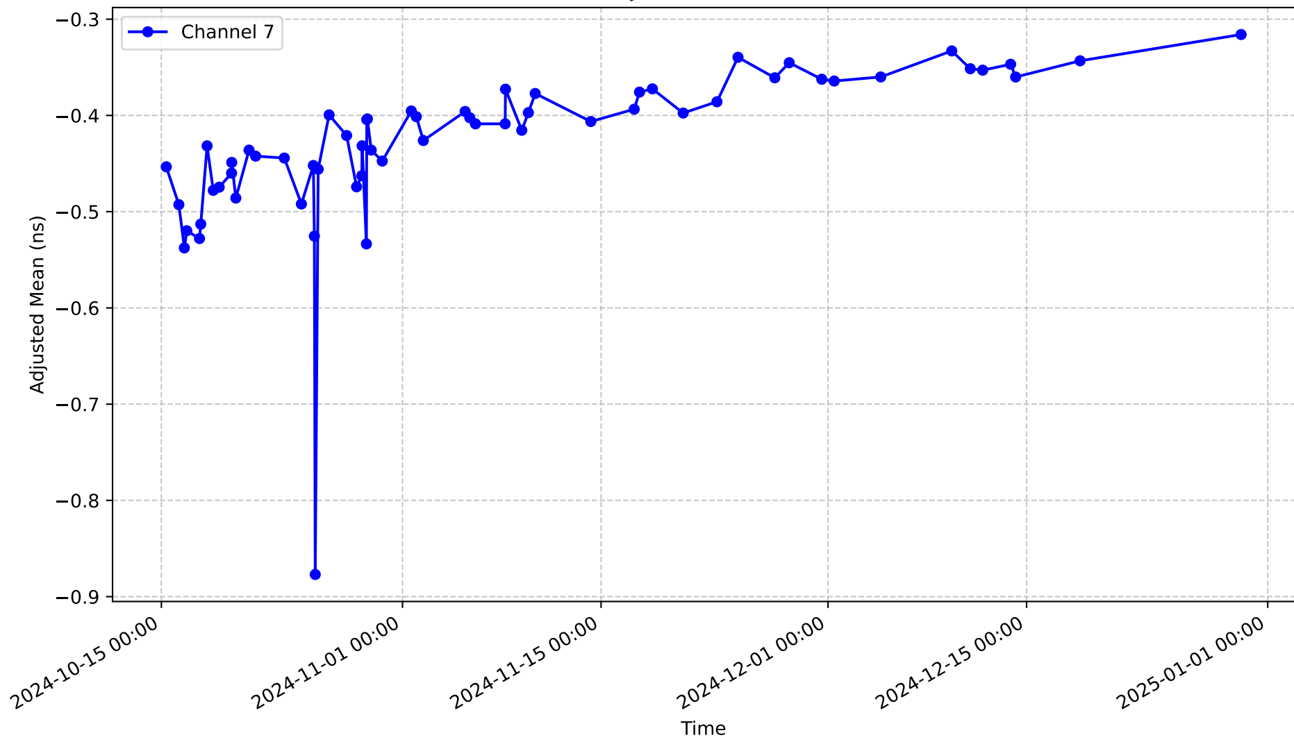
Channel 7 - Adjusted Mean Value Variation
