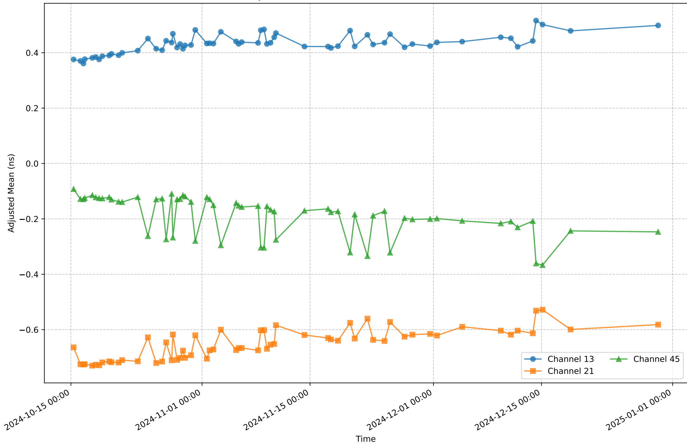
Adjusted Mean Variation for Channels \equiv 5 \bmod 8
