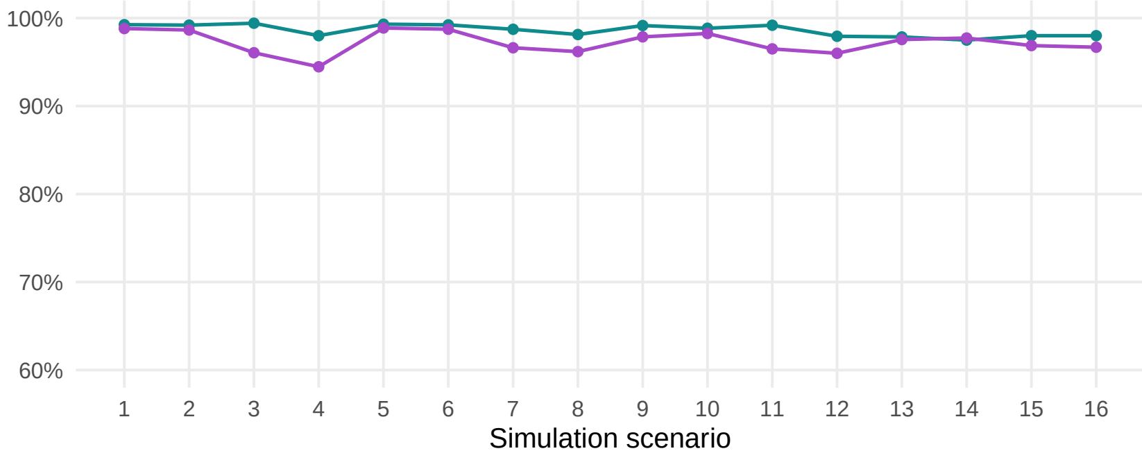
Pattern agreement vs PsN-SCM
