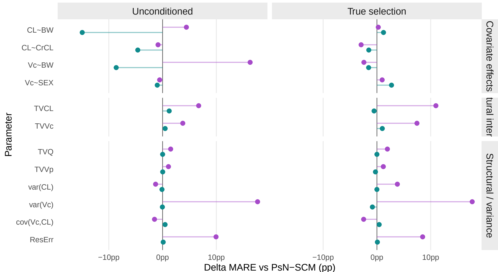
Difference in MARE vs PsN-SCM, scenario 16 (linCmt, N = 80). Left of 0 = more accurate than PsN-SCM; right = less accurate.
