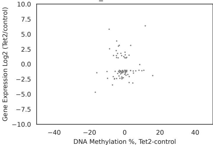
Preleukemia_Tet2VsControl PCC:0.056
