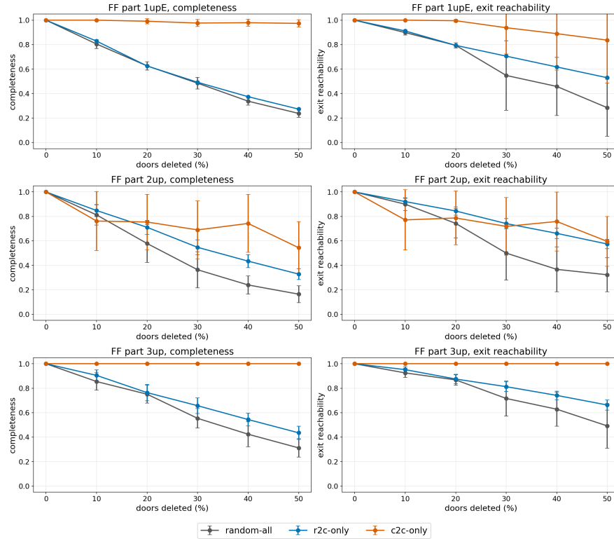
Fig. 3. Connectivity under door deletion for three floor sections. Random deletion and room-to-corridor deletion degrade completeness steadily because each room is single-homed through one access door. Corridor-to-corridor deletion barely moves two of the floors and bites on the third, which motivates the per-door analysis.
