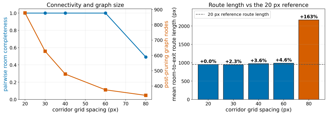
Fig. 5. Corridor density trade-off on first-floor section A. The left panel shows that completeness holds from 20 to 60 pixels and collapses at 80, while graph size grows steeply toward dense spacing. The right panel shows the mean room-to-exit route length per spacing, and the label above each bar gives its change relative to the 20-pixel reference.
