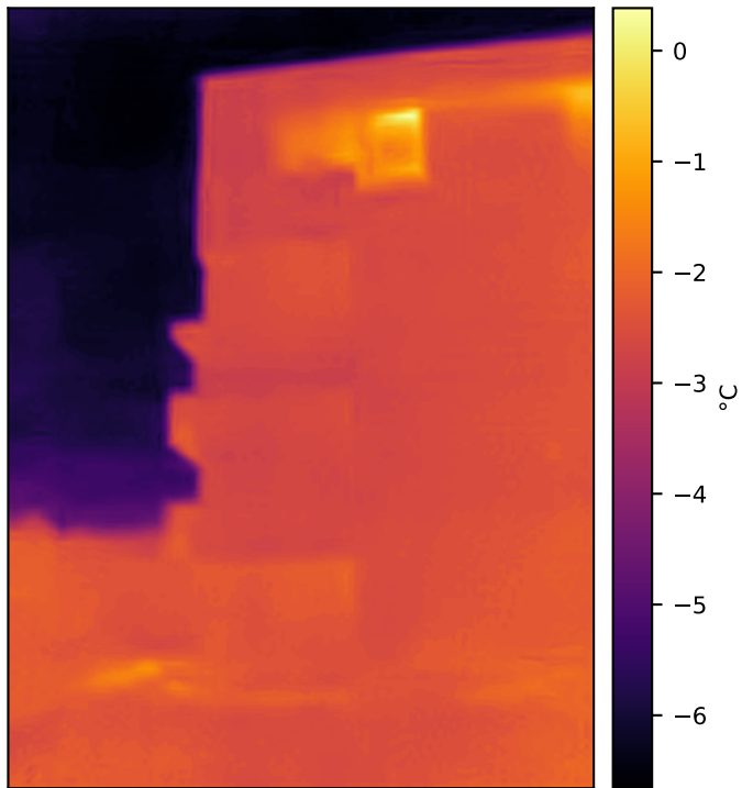
building-sunrise — calibrated surface temperature
