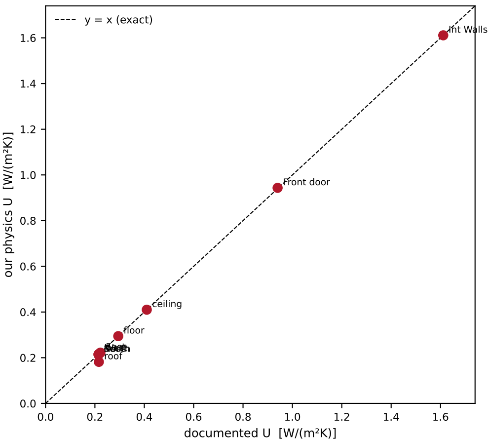
Twin Houses — U-value validation U-MAE 0.0042 W/(m 2 K) over 9 real elements
