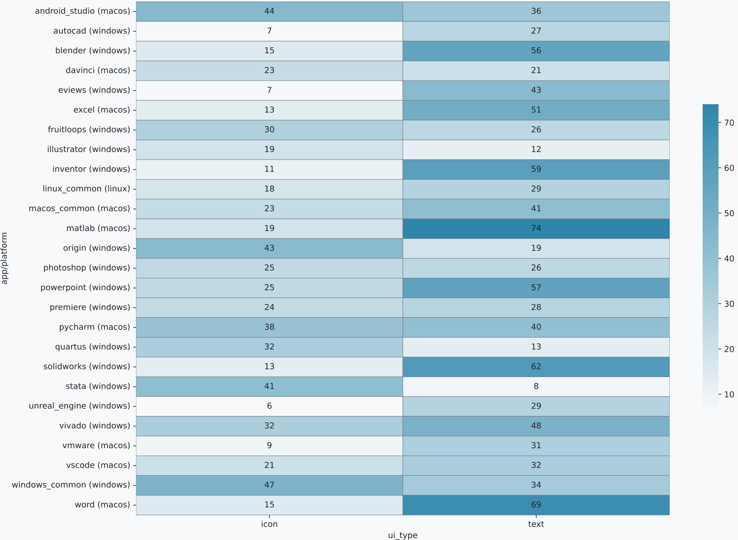
ScreenSpot-Pro Examples Count: app/platform x ui_type
