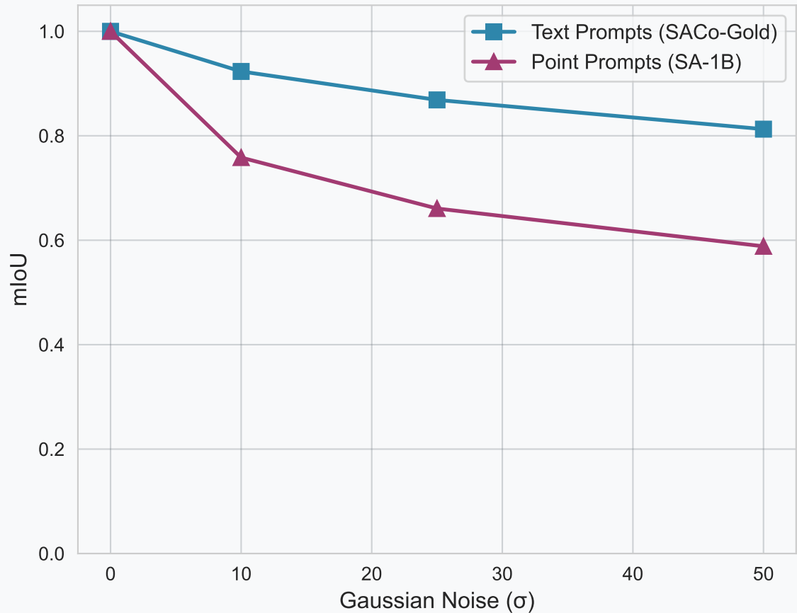
Visual Noise Robustness
