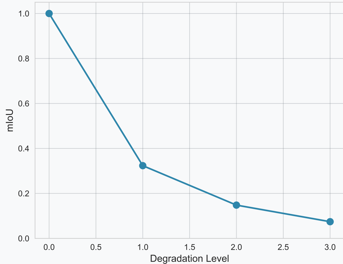
Linguistic Fragility (SACo-Gold)
