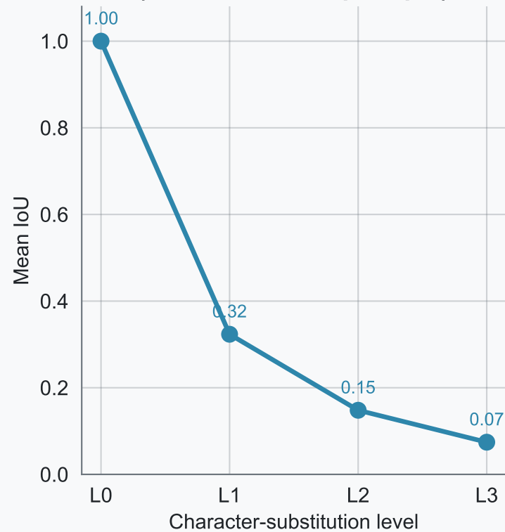
(A) Linguistic Fragility (SACo-Gold, text prompts)
