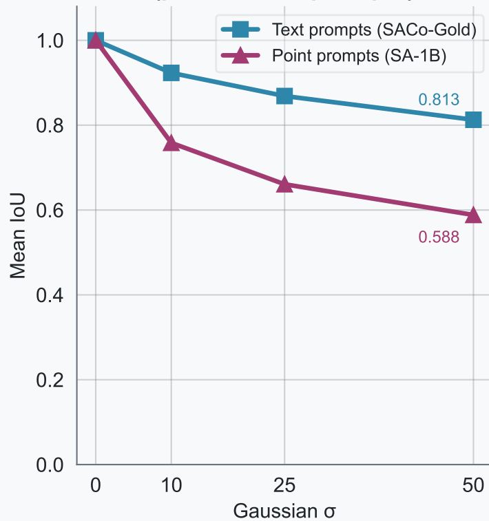
(B) Gaussian Noise Robustness (point vs text prompts)
