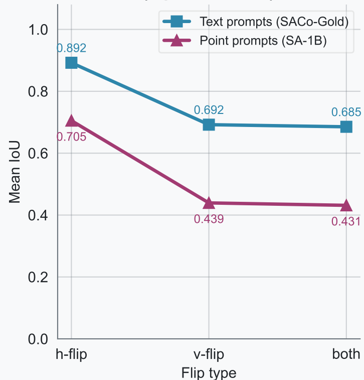
(C) Flip Equivariance (flip-back mIoU)
