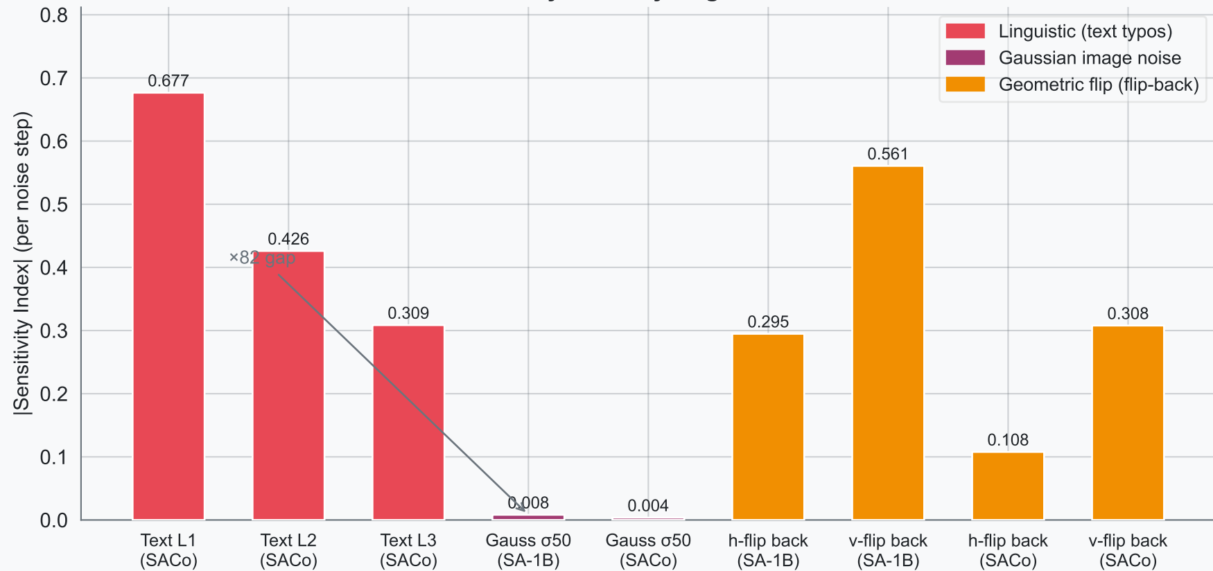
SAM 3 Sensitivity Index by Degradation Condition
