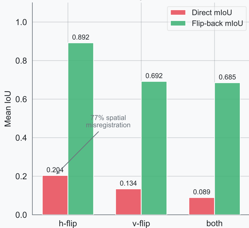
(B) SAcO-Gold — Text Prompts Direct vs Flip-back mIoU
