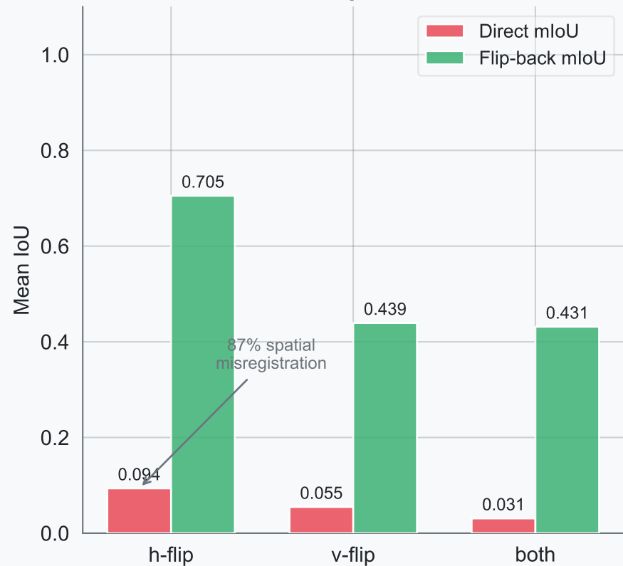
(A) SA-1B — Point Prompts Direct vs Flip-back mIoU
