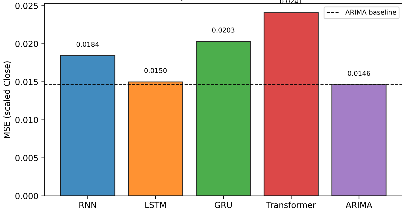
Mean Squared Error — all models
