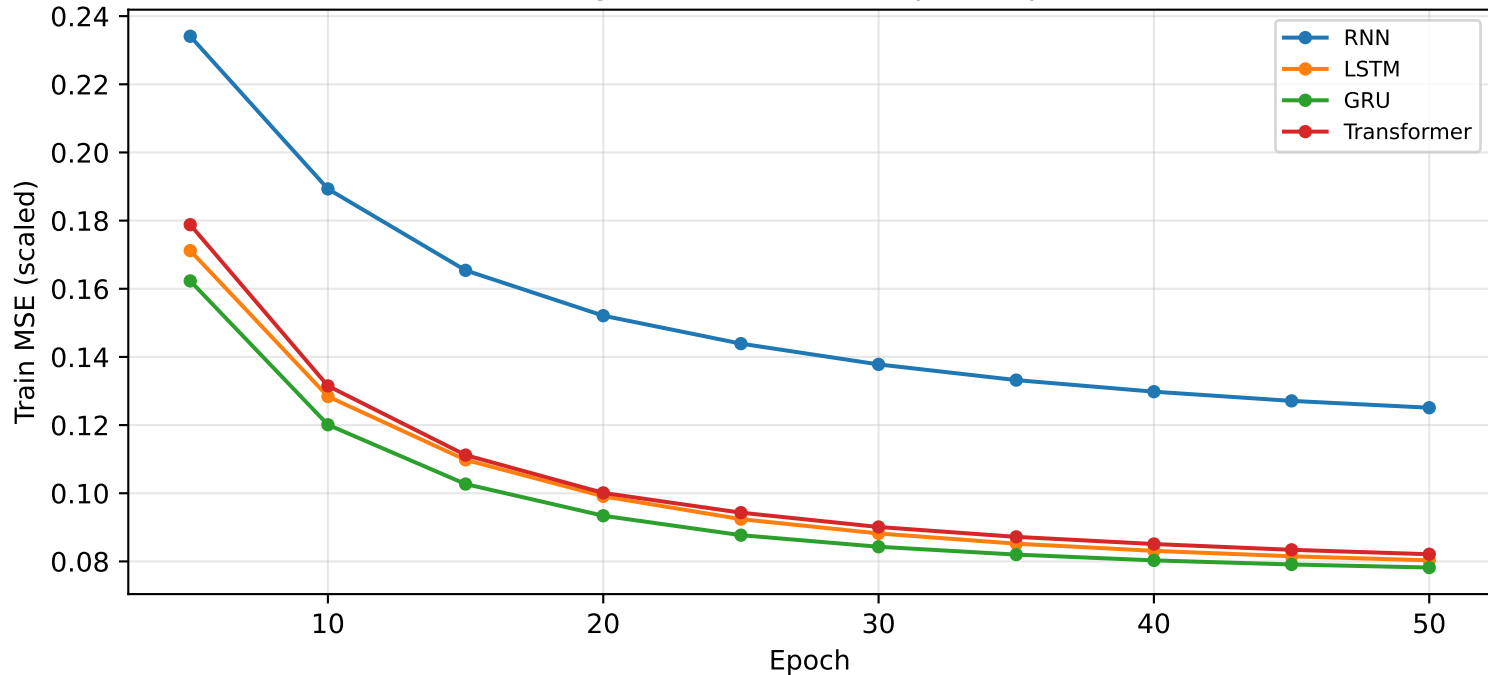
Training Loss Curves (MSE per 5 epochs)
