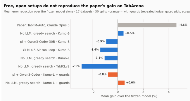
Figure 1. Mean gain of the searched pipeline over the frozen model alone on the 17 small TabArena datasets, all 30 official splits. No free setup reproduces the paper.
