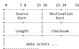
User Datagram Header Format
