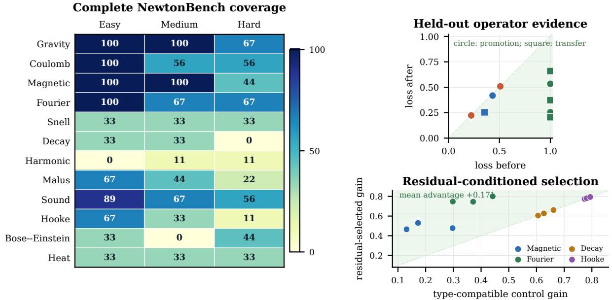
Figure 4: Complete NewtonBench coverage and the frozen language-growth audit. Left: exact symbolic accuracy over all 324 task configurations; each cell averages three law versions and three system variants. Upper right: executable loss before and after accepted operators on held-out promotion and disjoint transfer interfaces. Lower right: 12 paired evaluations compare the residual-selected family with a type-compatible control under identical fitting and test-time compute; points above the diagonal favor residual conditioning.
